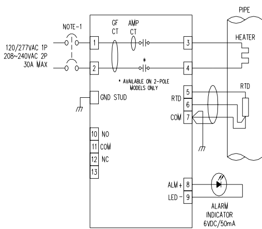
Figure 3.1 Thermostat Replacement
