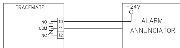
Figure 3.2 Alarm Annunciator
